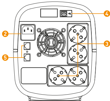
Back Panel
