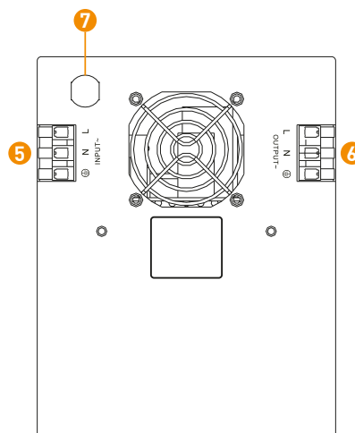
Back Panel
